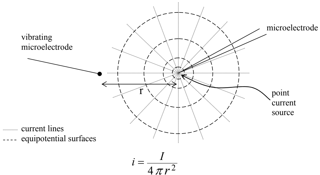
Figure 2. Schematic representation of microelectrode tip used as a point current source for calibration. The equation gives the current i that should be measured at a distance r from the source of current I [17].
