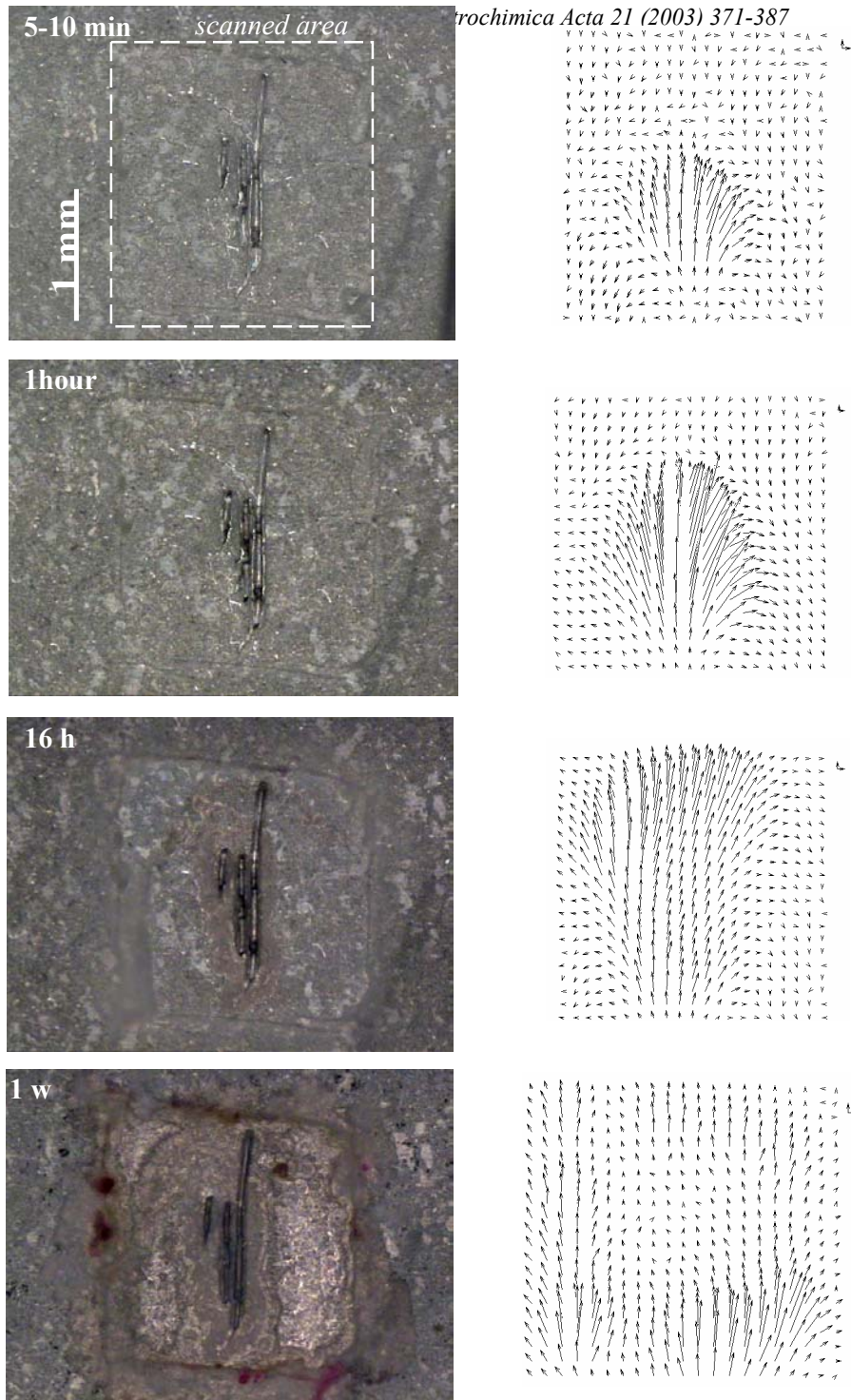
Figure 6. Optical images and current density maps of electrogalvanized steel with a defect exposed to 0.1 M NaCl, at various immersion times. On the top right of each map a two vectors scale corresponds to 10 \mu\text{Acm}^{-2} in each direction.
