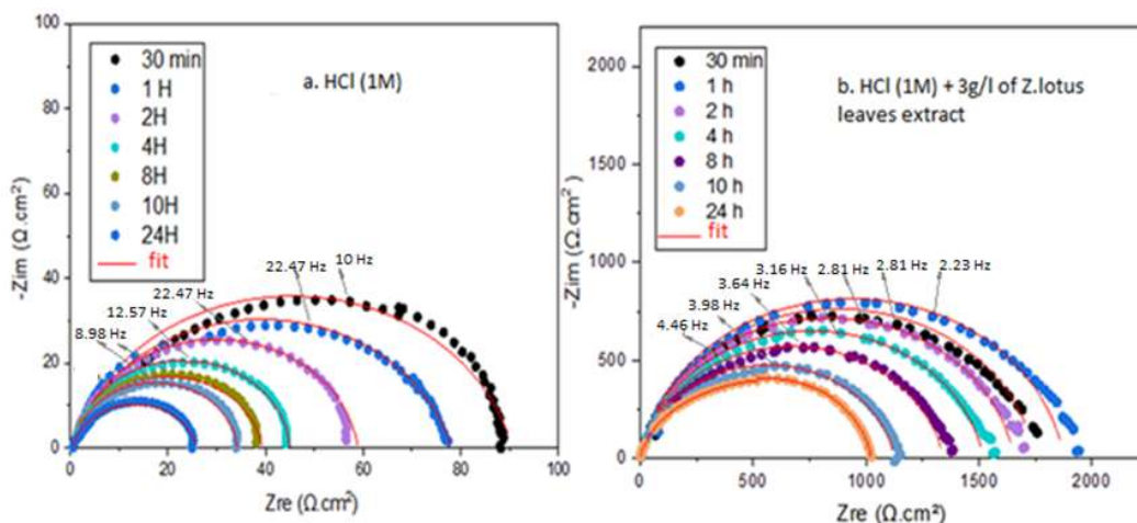
Figure 7. CS Nyquist plots in: a) 1 M HCl and b) 1 M HCl + 3 g/L of ZL extract, with different times of immersion, at 293 K.
