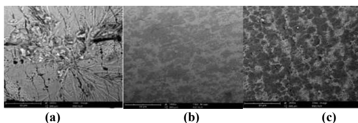
Figure 5: Images obtained from SEM for Fe corrosion in: (a) pure 1 M HCL; (b) with 1.0 g/L SAA; and (c) with 7.5 g/L SAA.
