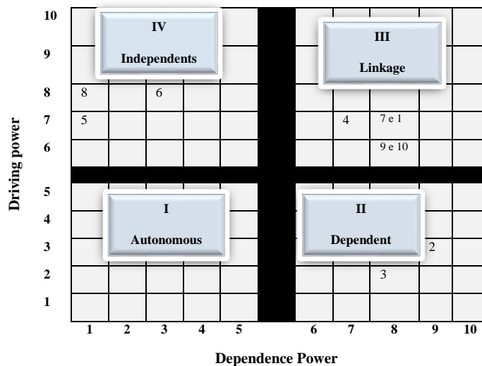
Figure 2. Clustering diagram.
