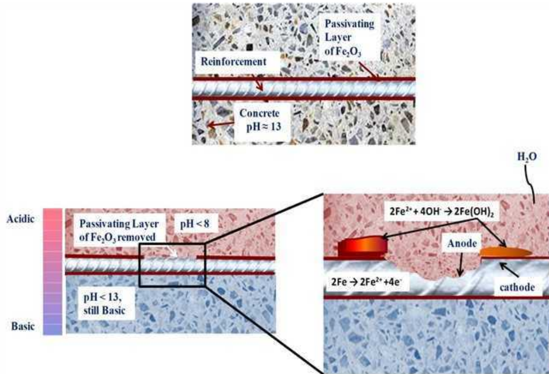
Figure 2: Depassivation of protective oxide film due to Cl^- ingress.
