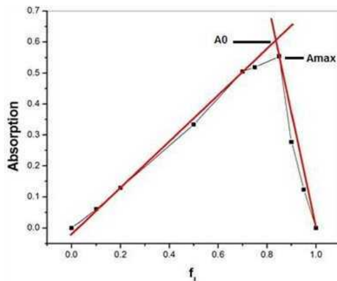
Figure 6: Job's diagram for Cd-Na-DDTC complex in 0.1 M NaClO 4 ( \lambda_{max} = 300 nm).
