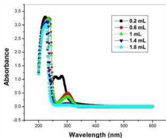
Figure 5: Cd-Na-DDTC absorption spectra in a solution with decreasing Na-DDTC, increasing CS and constant total C_t in 0.1 M \text{NaClO}_4 , at 298 \pm 0.1 K.
